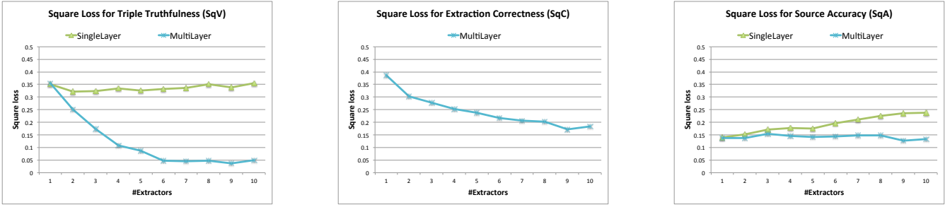
Figure 3: Error in estimating V_d , C_{wdev} and A_w as we vary the number of extractors in the synthetic data. The multi-layer model has significantly lower square loss than the single-layer model. The single-layer model cannot estimate C_{wdev} , resulting with one line for SqC.
