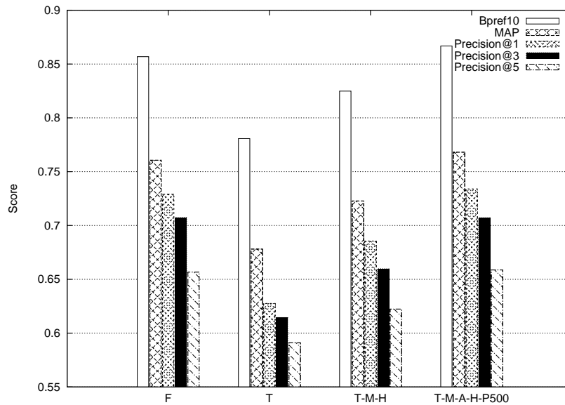
Fig. 9. The scores of various text summarization options for Dataset 1. F corresponds to the full-page, M to the meta data, to H the headings sections of the page, A to the anchor text of the page’s outgoing links, and P500 to the page’s first 500 bytes. The results are with classification.
