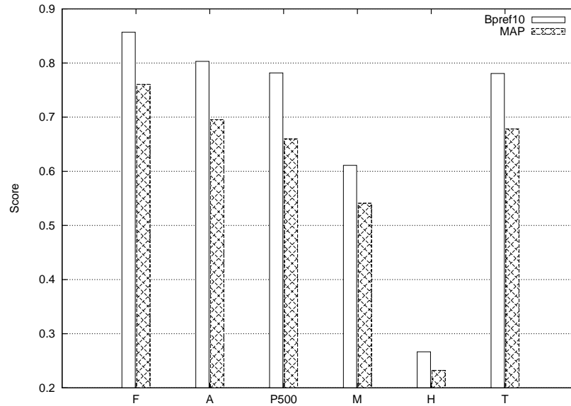
Fig. 11. The scores of individual page fragments for Dataset 2. The values in the x -axis are sorted in decreasing order of average length. F corresponds to the full-page, A to the anchor text of the page's outgoing links, P500 to the page's first 500 bytes, M to the meta data, H the headings sections, and T to the page's title. The results are with classification.
