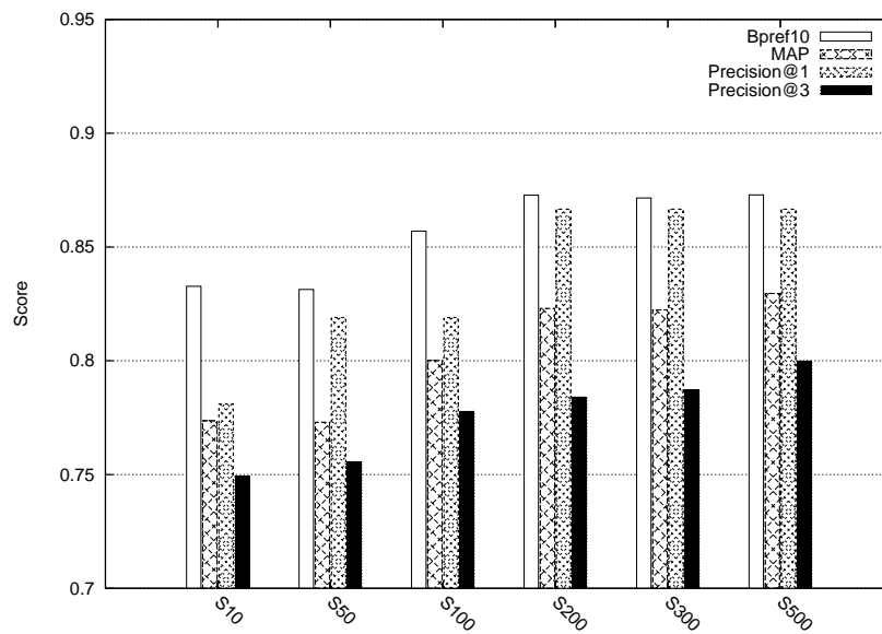
Fig. 19. Performance of the MEAD summarization as the length of the summaries increases for Dataset 1. The values in the x -axis (denoted by S_x ) correspond to the number of words requested. The results are with classification.
