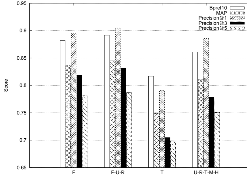
Fig. 8. The scores of various text summarization options for Dataset 1. F corresponds to the full-page, U to the page’s URL, R to the referrer page’s URL, M to the meta data, and H to the headings sections of the page. The results are with classification.
