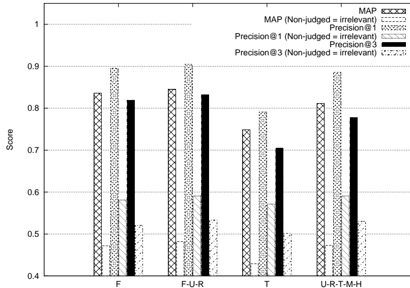
Fig. 16. Comparison of scores when non-judged ads are ignored and when they are taken into account and considered as irrelevant in Dataset 1. F corresponds to the full-page, U corresponds to the page's URL, R to the referrer page's URL, T to the page's title, M to the meta data, and H to the headings sections of the page. The results are with classification. We can see that the two sets of scores are highly correlated, in particular, the relative order of the scores is almost always the same, whether we take non-judged ads into account or not.
