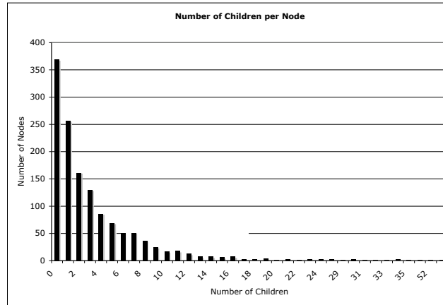
Fig. 3. Taxonomy statistics: fanout of non-leaf nodes
