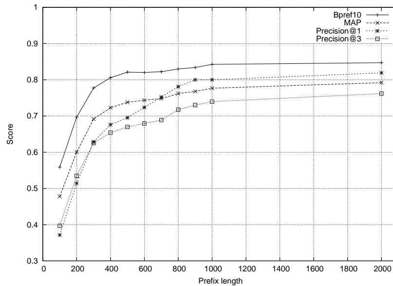
Fig. 12. The scores with prefixes of various length for Dataset 1. The values in the x -axis (denoted with P_x in the text) correspond to the length in bytes of the prefix used. The results are with classification.
