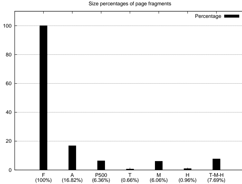
Fig. 7. Size percentages of various segments and their combinations for Dataset 2. F corresponds to the full-page, M to the meta data, H to the headings sections of the page, A to the anchor text of the page's outgoing links, and P500 to the page's first 500 bytes
