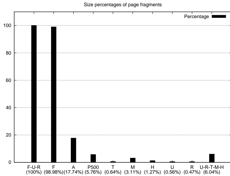
Fig. 6. Size percentages of various segments and their combinations for Dataset 1. F corresponds to the full-page, U to the page's URL, R to the referrer page's URL M to the meta data, H to the headings sections of the page, A to the anchor text of the page's outgoing links, and P500 to the page's first 500 bytes
